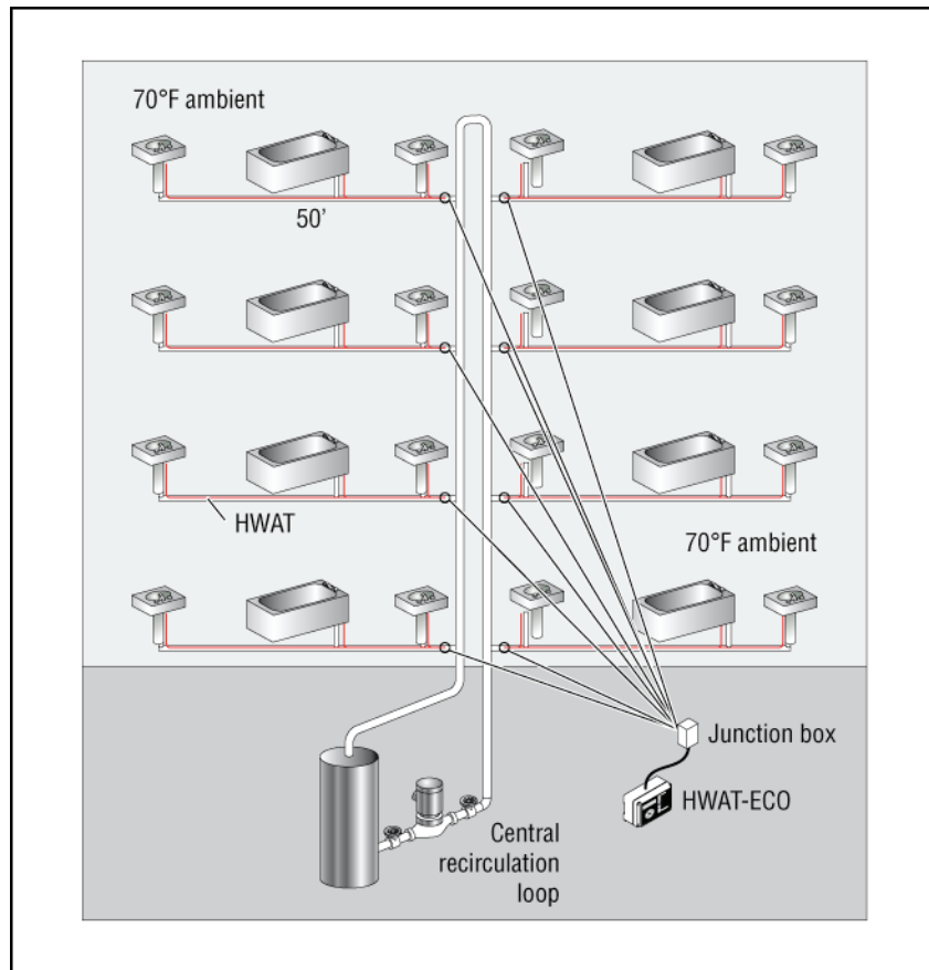
Figure 1: Generic Hybrid HWAT System
